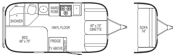
SAFARI 19 Bambi - with sofa option
